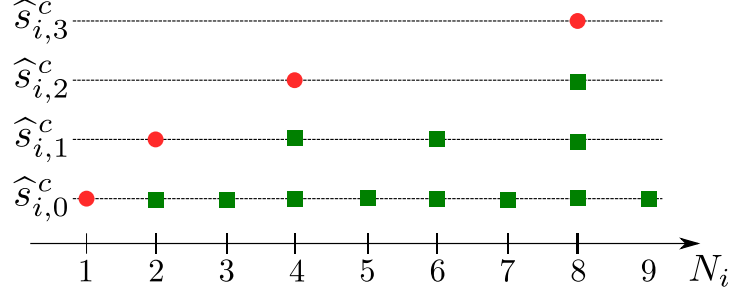
Figure 3: Illustration of the functioning of EFF-FEWA. The red circles denotes the number of pulls of arm i at which a new estimate \widehat{S}_{i,j}^c is created corresponding to a window h = 2^j , while the green boxes indicate the number of pulls for which \widehat{S}_{i,j}^c is updated with the last 2^j samples.
