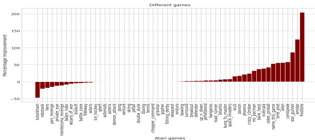
Figure 6: Relative improvement of retrieval-augmented R2D2 vs vanilla R2D2 on different Atari games, measured by human normalized score. We report the average score from 3 seeds per method and per game.
