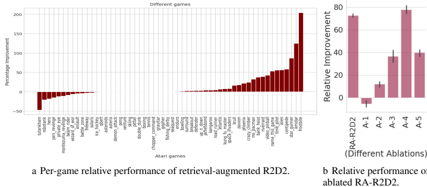
Figure 2: (a) Relative percentage improvement in mean human normalized score of retrieval-augmented R2D2 vs vanilla R2D2 on different Atari games, measured by human normalized score. We report the average score from 3 seeds per method and per game. (b) Relative percentage improvement of ablated RA-R2D2 versus baseline R2D2 for 5 ablations on 10 Atari games. Black lines show standard deviations from 3 seeds.
