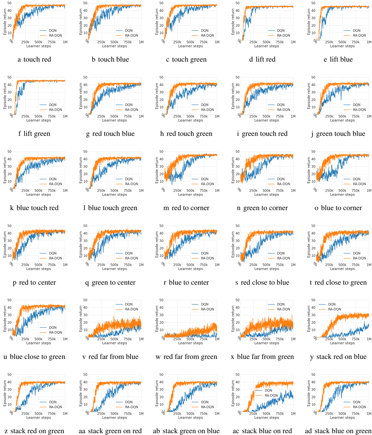
Figure 9: Multi-task offline RL with a task-specific retrieval dataset. Evaluation performance for RA-DQN (orange) and baseline DQN (blue) when training on all 30 gridroboman tasks with a single agent. Curves show the performance of each agent (averaged over 3 seeds) when running that agent online in the environment on the specified task.
