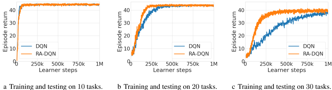
Figure 3: Gridroboman: Multi-task offline RL with a task-specific retrieval dataset. Average episode return vs. learner steps for the multi-task gridroboman environment when training and evaluating on 10, 20, and 30 tasks. With fewer tasks (a), the baseline DQN agent (blue) and the retrieval-augmented DQN agent (orange) perform identically; however, when the number of tasks increases (b, c), the retrieval-augmented agent learns much more effectively than the baseline DQN agent. Results are the average of 3 seeds for each method. Curves for individual tasks are shown in the appendix (Figure 9).
