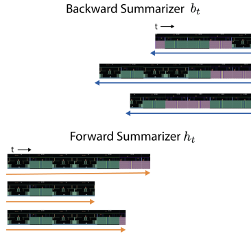
Figure 5: Each trajectory in the retrieval batch is summarized via a forward and a backward running parametric structured model (Transformers or slot based recurrent network). Each state in the trajectory is represented by a (h_t, b_t) tuple where h_t represents the summary of the past and b_t represents the summary of the future with that trajectory.
