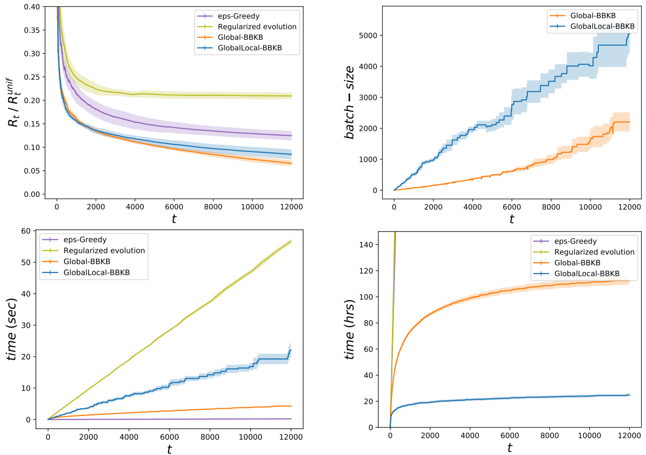
Figure 7: From left to right and from top to bottom: regret ratio, batch-size, time without experimental costs and total runtime on the NAS-bench-101 dataset, with Gaussian kernel with bandwidth 100
