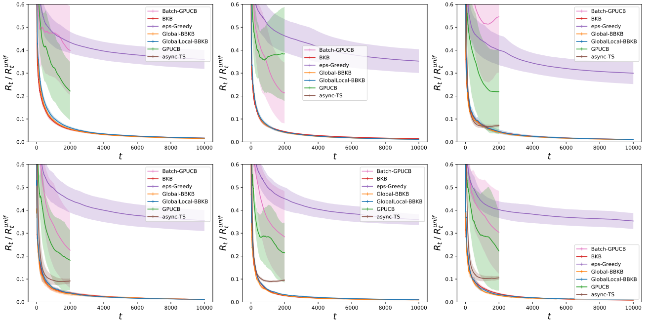
Figure 5: Regret ratio for the Abalone dataset, with Gaussian kernel with, from left to right and from top to bottom, badwidths equal to 5, 7.5, 10, 12.5, 15, 17.5
