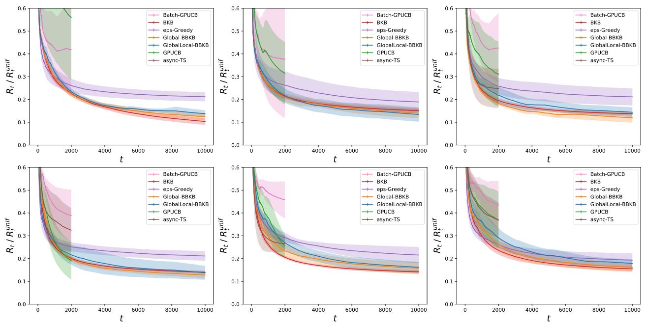
Figure 6: Regret ratio for the Cadata dataset, with Gaussian kernel with, from left to right and from top to bottom, badwidths equal to 5, 7.5, 10, 12.5, 15, 17.5
